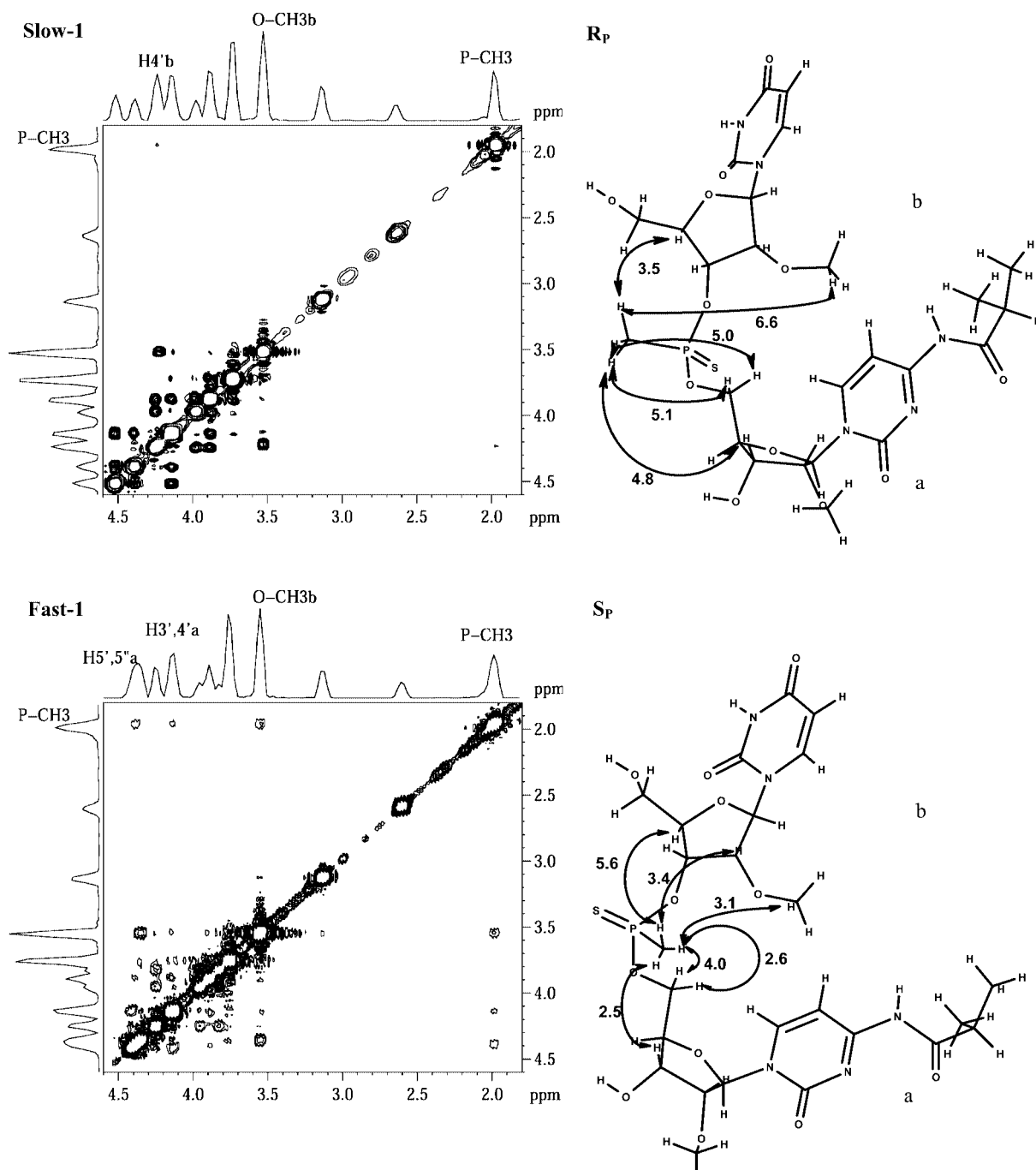
Figure 2. ^{31}\text{P} NMR decoupled ROESY spectra of Slow-( R_P )-1 (a) and Fast-( S_P )-1 (b) registered at 25 °C
