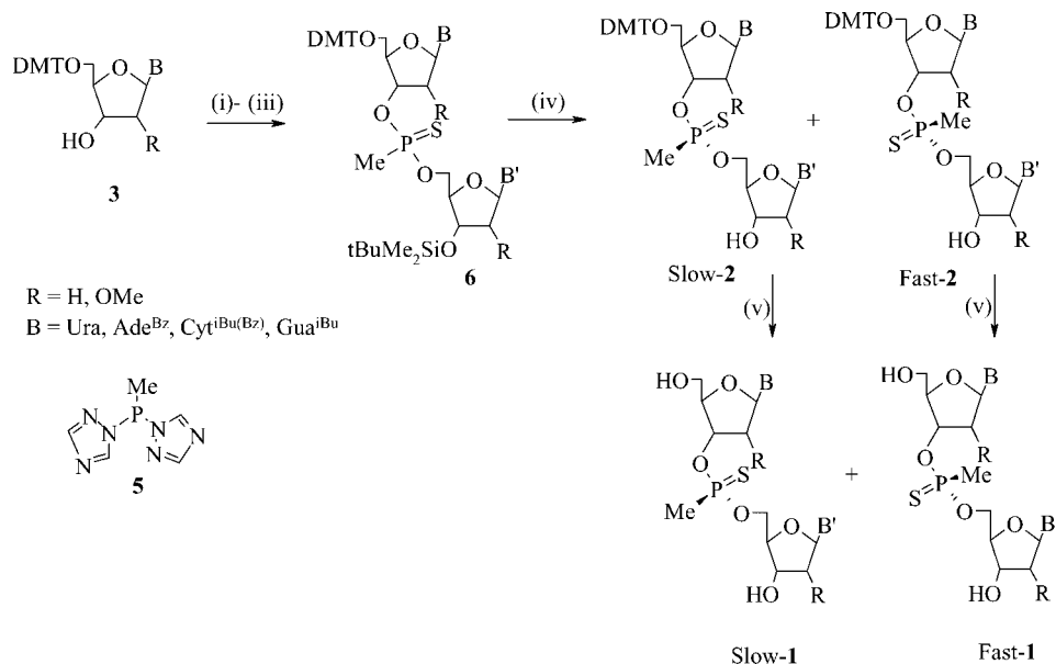
Scheme 1. Reagents and reaction conditions: (i) dropwise addition of 3 to 5 , ice bath, 45 min; (ii) 3'-protected nucleoside 4 in THF, room temp, 1.5 h; (iii) elemental sulfur, room temp., overnight, followed by aqueous workup, precipitation; (iv) Et 3 N·3HF/Et 3 N in THF, followed by silica gel column chromatography; (v) 2% dichloroacetic acid, CH 2 Cl 2 , 10 min, room temp.
