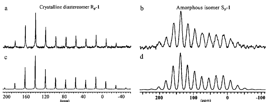
Figure 4. Room-temperature ^{31}\text{P} CP/MAS spectra of ( R P )- 1 , crystallized from ethanol (a), and amorphous ( S P )- 1 (b), together with the corresponding WINMAS program simulations (c and d)
