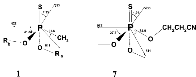
Figure 5. Principle elements of chemical shift tensors for compounds 1 and 7
