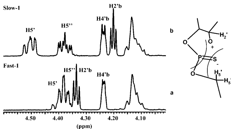
Figure 3. Expanded region of the H5' protons for ( R P )- 1 (Slow) and ( S P )- 1 (Fast)
