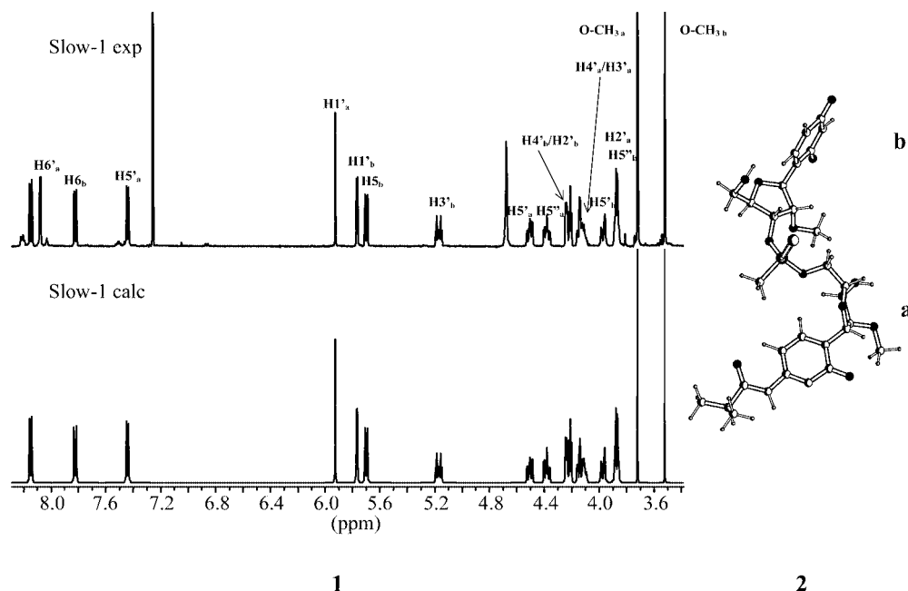
Figure 1. (1) Spectrum of Slow-1 recorded in \text{CDCl}_3 and the theoretical spectrum modelled with the WINDAISY program; [21] (2) the 3D structure of diastereomer Slow-1 obtained by the PM3 semiempirical method [22]
